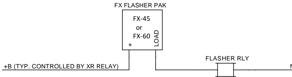
TYPICAL WIRING HOOKUP
